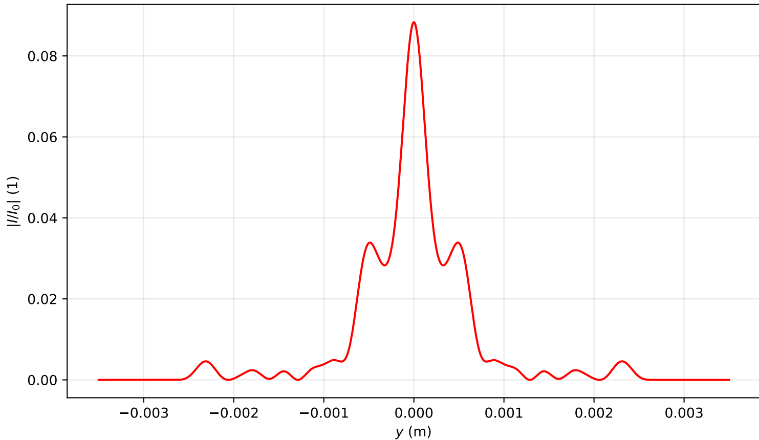
Intensity profile I(x=0, y, z=3.981)/I_0 , P_{in}=8.0P_{cr} , artificial time
